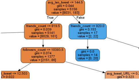
Fig. 17. Top portion of the decision tree0.
