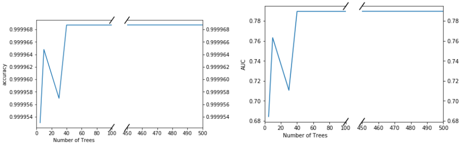
Fig. 16. (Left) Accuracy with different number of trees and (Right) AUC with different number of trees for the random forest algorithm.
