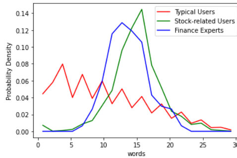
Fig. 8. The distribution of the average number of words per tweet when the number of bins is 20.
