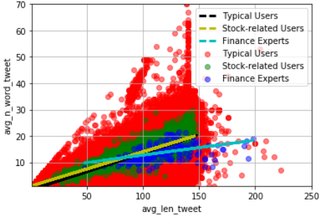
Fig. 14. The distribution of users in terms of avg_len_tweet and avg_n_word_tweet . Each dot represents one user. There are three trendlines representing the three user groups, respectively. Slope for each trendline: Typical: 0.14, Stock-related: 0.13, Expert: 0.056.
