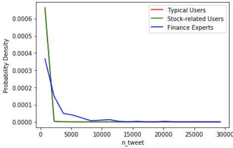
Fig. 1. The distribution of n_tweet for the three user groups. Typical users and stock-related users are almost identical and cannot be differentiated.
