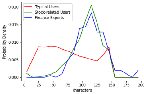
Fig. 6. The distribution of the average number of characters per tweet.
