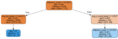
Fig. 19. Top portion of the decision tree25.
