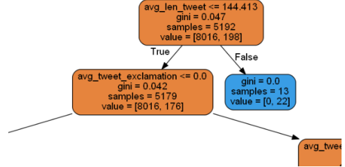
Fig. 18. Top portion of the decision tree15.
