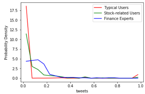
Fig. 12. The distribution of proportion of tweets containing “?”.
