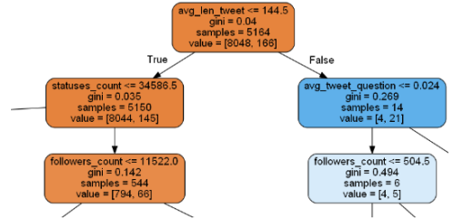
Fig. 20. Top portion of the decision tree35.
