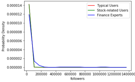
Fig. 4. The distribution of the number of followers.
