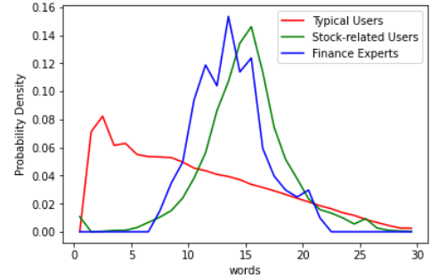
Fig. 7. The distribution of the average number of words per tweet.
