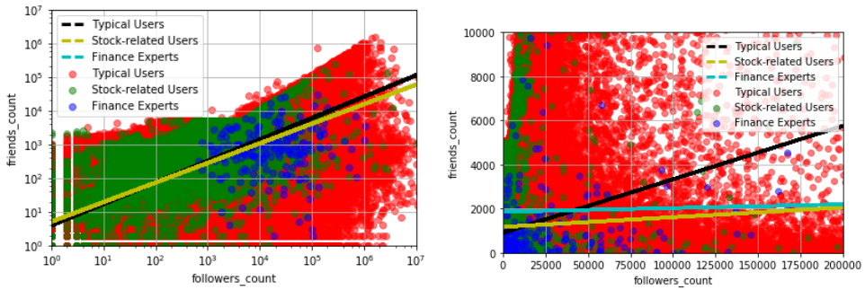
Fig. 13. (Left) The distribution of users in terms of friends_count and followers_count. Each dot represents one user. (Right) The distribution set with a smaller focus region. There are three trendlines representing the three user groups, respectively. Slope for each trendline: Typical: 0.0243, Stock-related: 0.0044, Expert: 0.0017.
