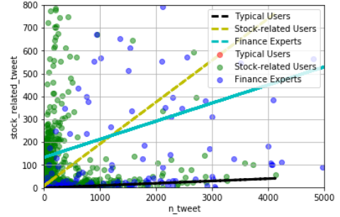
Fig. 15. The distribution of users in terms of n_tweet and stock_related_tweet . Each dot represents one user. Because the quantity of n_tweet and stock_related_tweet in typical users are much smaller than stock-related users and experts, the red spots are hardly seen in this figure. However, we can still see there are three trendlines representing the three user groups, respectively. Slope for each trendline: Typical: 0.01, Stock-related: 0.183, Expert: 0.079.
