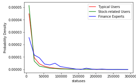
Fig. 3. The distribution of statuses_count.
