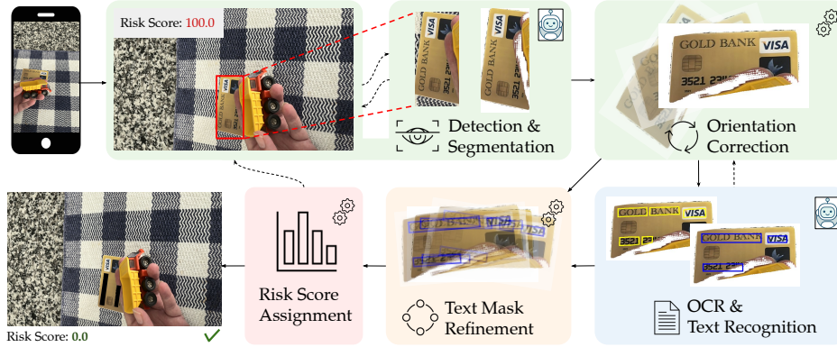
Figure 3: Multi-agent Collaboration System. Given an input image, the first agent [👁️] detects, localizes, and segments the private object. Next, a second agent [🔄] evaluates a set of angles to correct the object’s alignment. A third set of agents processes the aligned object [📄] for OCR, text recognition, and category assignments. Then, text mask refinement [🔍] is performed to map the fine-grained elements back onto the original image. Finally, the system assigns risk scores [📊] to each detected region and applies masking accordingly.
